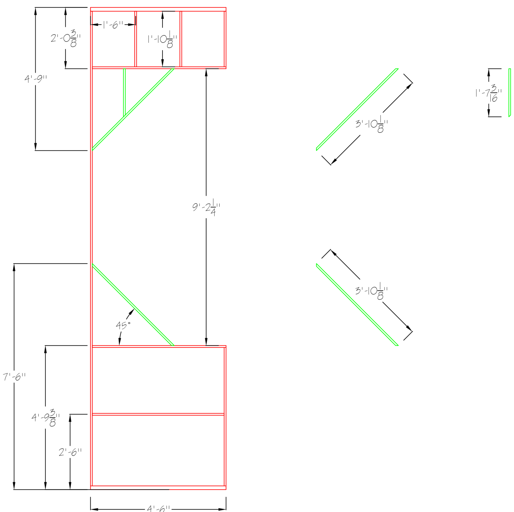
Front View C - without Planking
