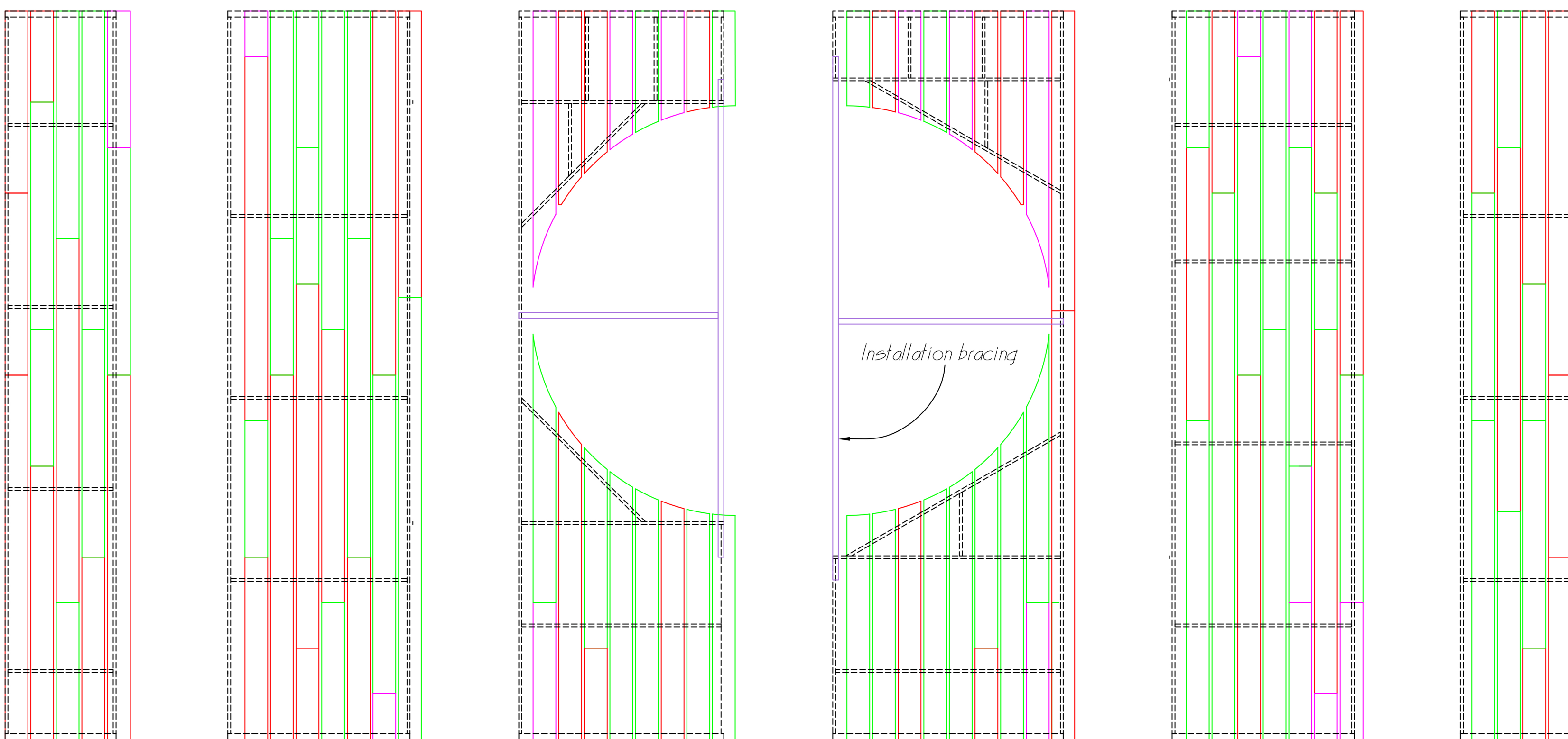
Front View - Plank breakdown
